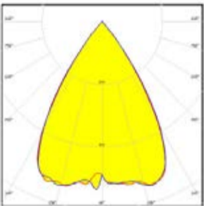
~65° extra wide beam. Variant with diffused lenses.
