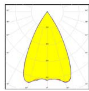
~65° wide beam
