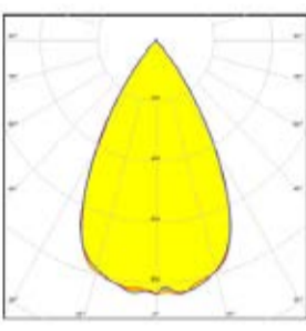
~65° wide beam. Variant with diffused lenses.
