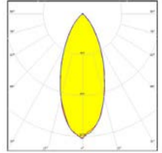
~65° extra wide beam. Variant with diffused lenses.
