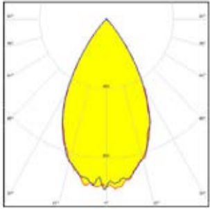
~55° wide beam
