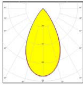
~55° wide beam. Variant with diffused lenses.
